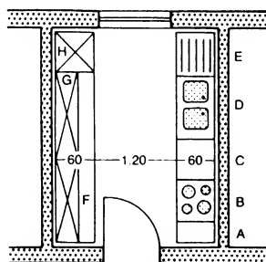
3 Effective kitchen workplace arrangement
